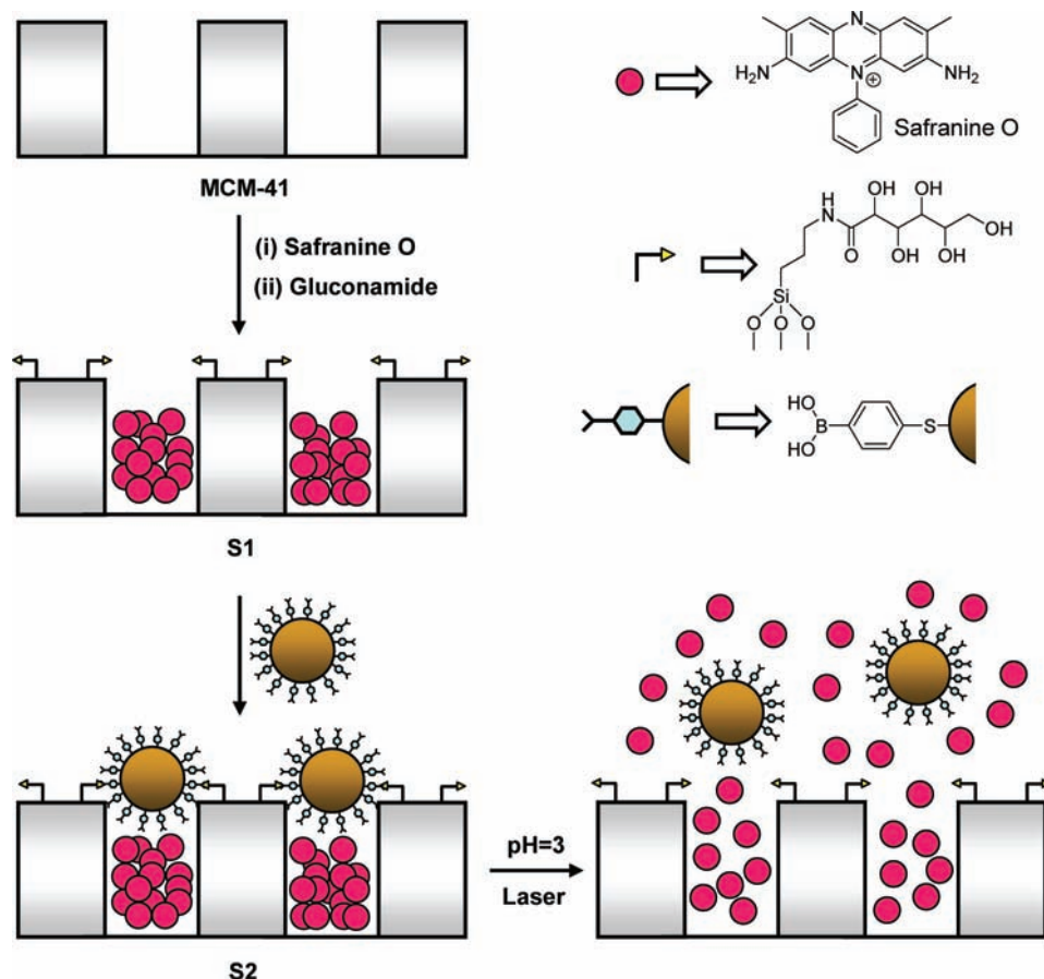
Scheme 1. Preparation of Solids S1 and S2 and the pH and Laser Light Triggered Release of the Entrapped Guest (the Dye Safranin O)
