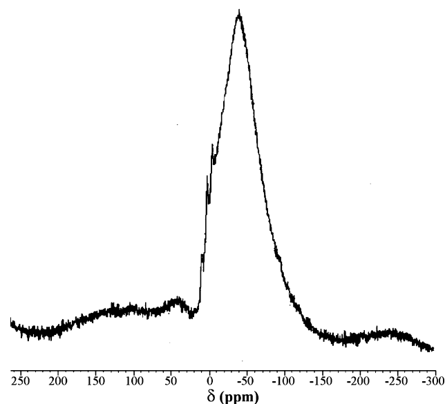
Figure 9. ^{11}\text{B} MAS NMR spectrum of S2 .
