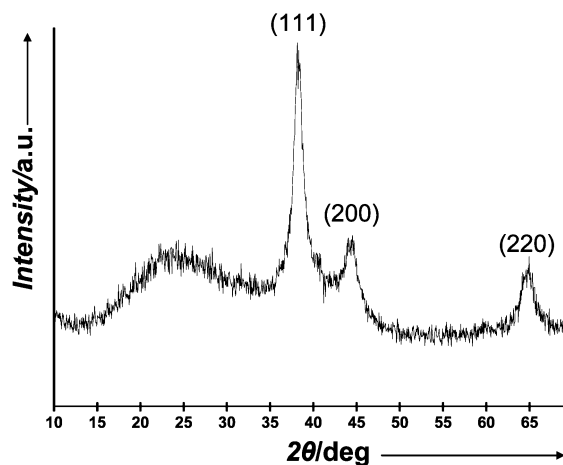
Figure 3. Powder X-ray patterns of the of the gold nanoparticles functionalized with boronic acid B-AuNPs. The broad peak at ca. 25° is due to the scattering of the glass amorphous support.
