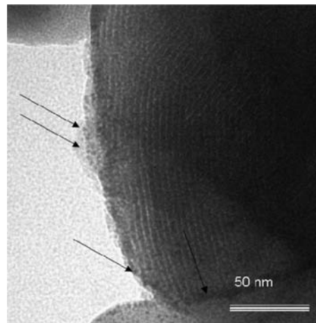
Figure 8. TEM image of the solid S2 showing the mesostructure. The arrows point to gold nanoparticles.
